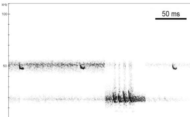
Figs. 122. Spectrogram of echolocation and social calls of Pipistrellus pipistrellus (Schreber, 1774): songflight of a male flying around a building in Jabla; advertising behaviour of P. kuhlii (Kuhl, 1817) was observed simultaneously at the same site.
