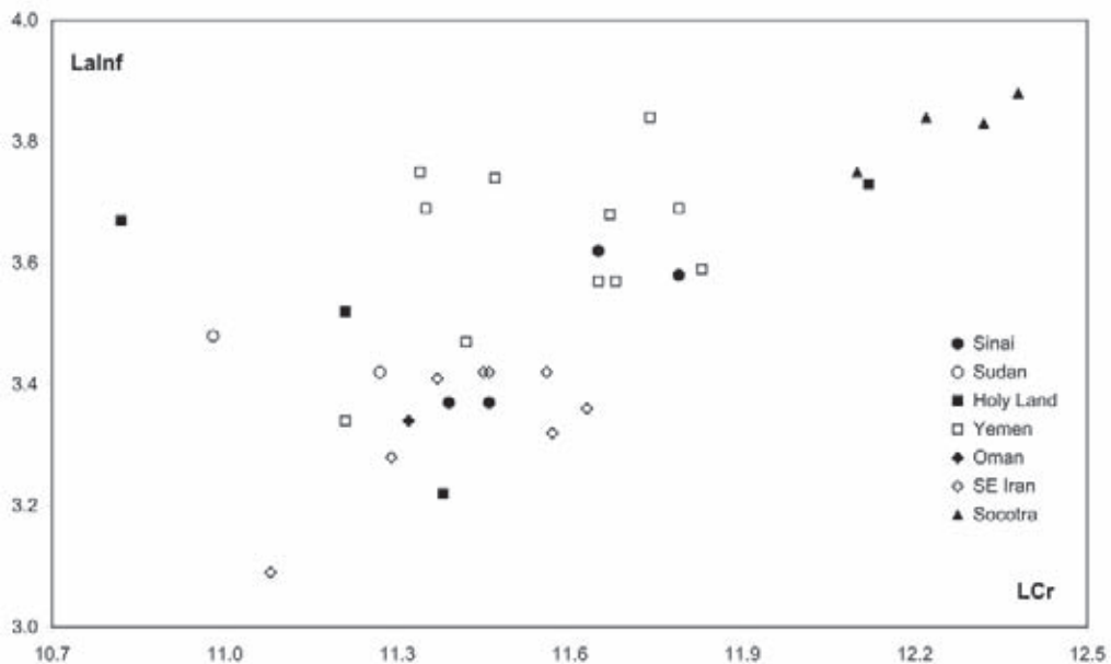
Fig. 35. Bivariate plot of examined Sinaitic and comparative samples of Hypsugo ariel (Thomas, 1904) and H. arabicus Harrison, 1979: greatest length of skull (LCr) against the infraorbital width of rostrum (LaInf).
