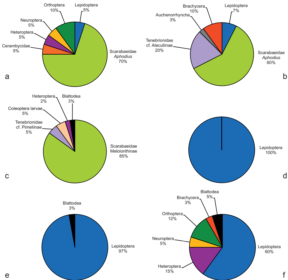
Fig. 16. Diet composition (percentage of volume): a – Rhinolophus clivosus Cretzschmar, 1830 (20 pellets collected from one individual); b – Hypsugo ariel (Thomas, 1904) (two digestive tracts analysed); c – Otonycteris hemprichii Peters, 1859 (two digestive tracts); d – Barbastella leucomelas (Cretzschmar, 1830) (two digestive tracts); e – Plecotus christii Gray, 1838 (seven digestive tracts); f – Tadarida teniotis (Rafinesque, 1814) (six digestive tracts).
