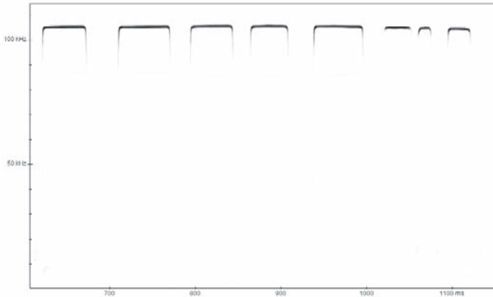
Fig. 24. Spectrogram of echolocation calls belonging most probably to Rhinolophus mehelyi Matschie, 1901. An individual flying around a water pit in the Ain Hudra Oasis.
