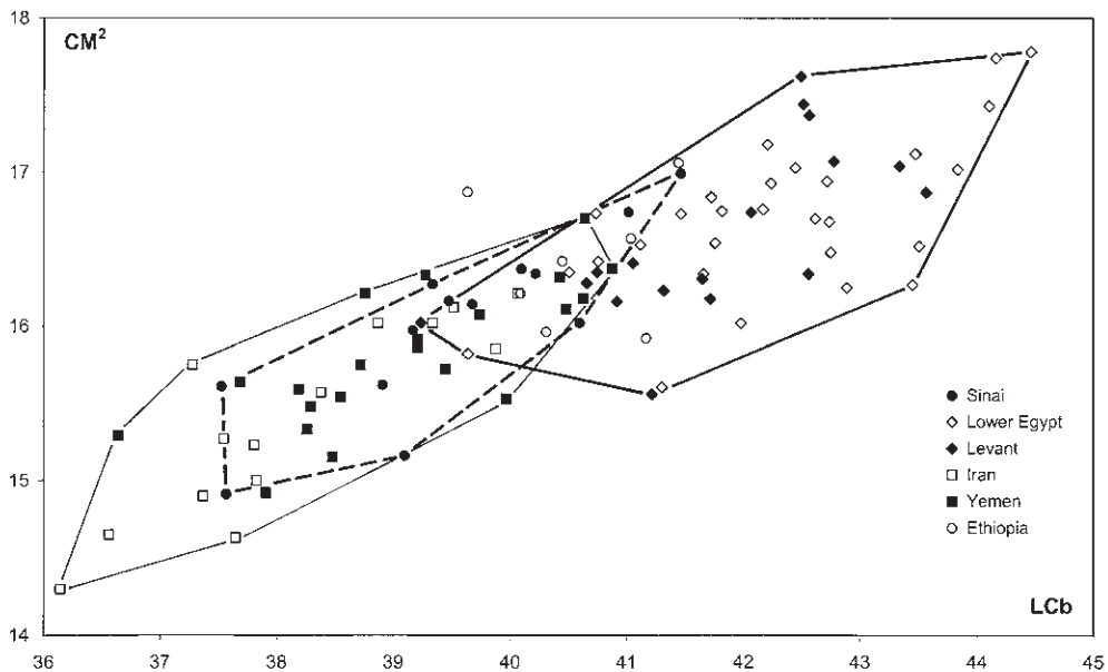
Fig. 8. Bivariate plot of examined Sinaitic and comparative samples of Roussettus aegyptiacus (Geoffroy, 1810): condylobasal length of skull (LCb) against the length of upper tooth-row (CM 2 ). Explanations: bold-lined polygon = samples from Lower Egypt and the Levant (n=46), i.e. of R. aegyptiacus aegyptiacus (Geoffroy, 1810); thin-lined polygon = samples from the southern parts of the Middle East (Iran, Yemen; n=35), i.e. nominally of R. aegyptiacus arabicus Anderson, 1902; dashed-lined polygon = samples from Sinai (n=13).
