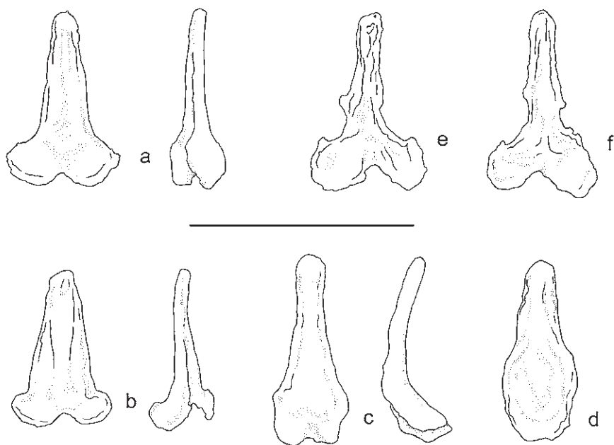
Fig. 59. Baculum preparations of Plecotini bats from Sinai a from comparative samples (distal epiphyses above; in pairs: left – dorsal view, right – lateral view): a – Barbastella leucomelas (Cretzschmar, 1830) (NMP 90521, Ain Hudra, Sinai); b – B. darjelingensis (Hodgson, 1855) (CUP CT84/253, Oš, Kirghizstan); c, d – B. barbastellus (Schreber, 1774) (c – SMM [unnumbered], Čížov, Czech Republic; d – NMP pb428, Čížov, Czech Republic); e, f – Plecotus christii petraeus ssp. n. (e – NMP 90499, Feiran, Sinai; f – NMP 92097, Wadi Rum, Jordan). Scale bar = 1 mm.
